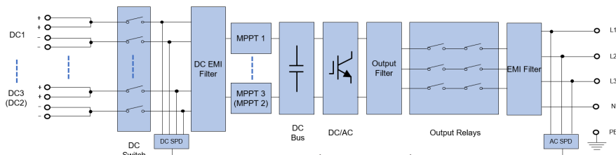
PV-30000S2-U (PV-22000S2-U)
