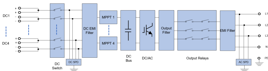
PV-50000S2-U
