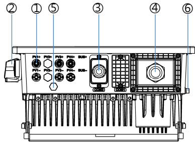
PV-15000S-U
